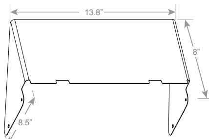
Glare Shield for HMPALDSR-403530L-3CCT HMPALDSR-403530L-3CCT-GS
