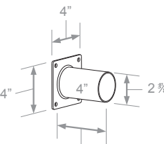
Wall Mount Bracket LEDMPALPRO-WMB
