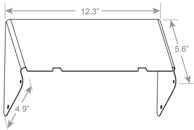
Glare Shield for HMPALDSR-242115L-3CCT HMPALDSR-242115L-3CCT-GS
